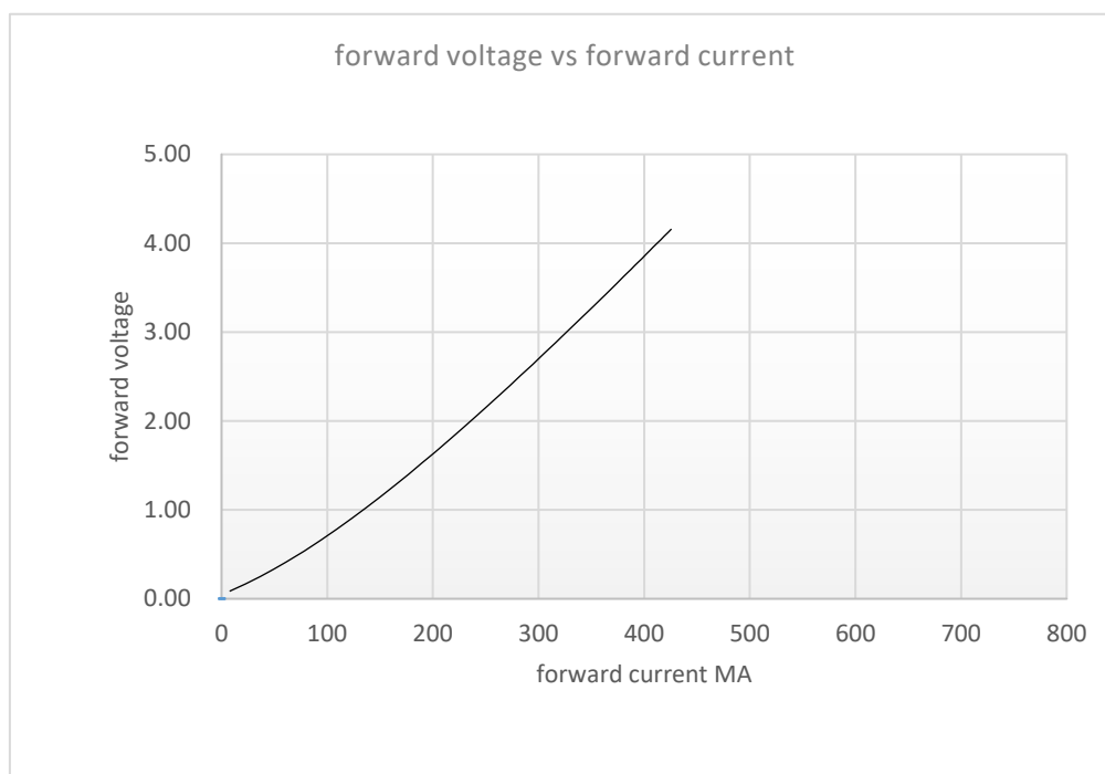
Figure 3. Typical forward current vs. forward voltage for R Tj=25°C.
