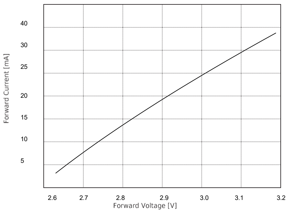
Typical forward current vs. forward voltage for at T_j=25^{\circ}\text{C} .
