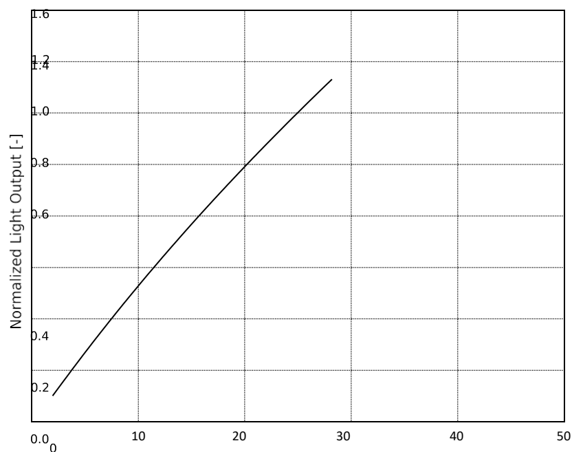
Figure 2. T Ambient temperature ( ^{\circ}\text{C} ) for at specified test current. T_j=25^{\circ}\text{C} .
