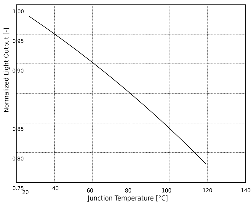
Figure 1. Typical normalized light output vs. junction temperature for at specified test current. T_j=25^{\circ}\text{C} .
