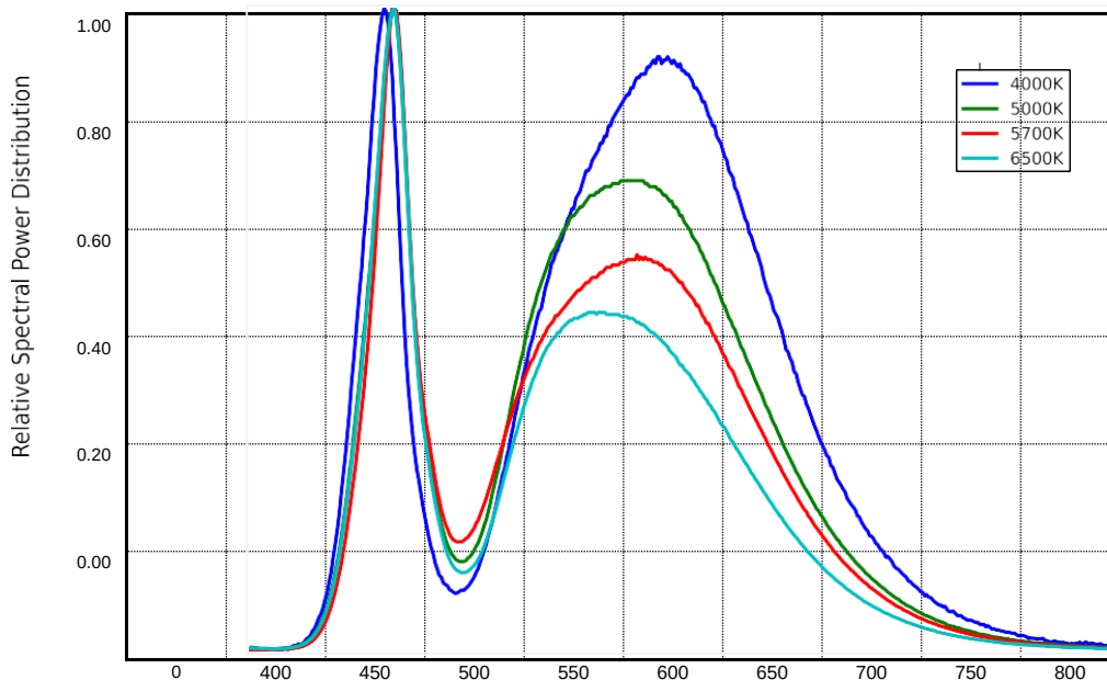
Figure 1: Typical normalized power vs. wavelength for Queendom at specified test current, T_j=85^{\circ}\text{C}
