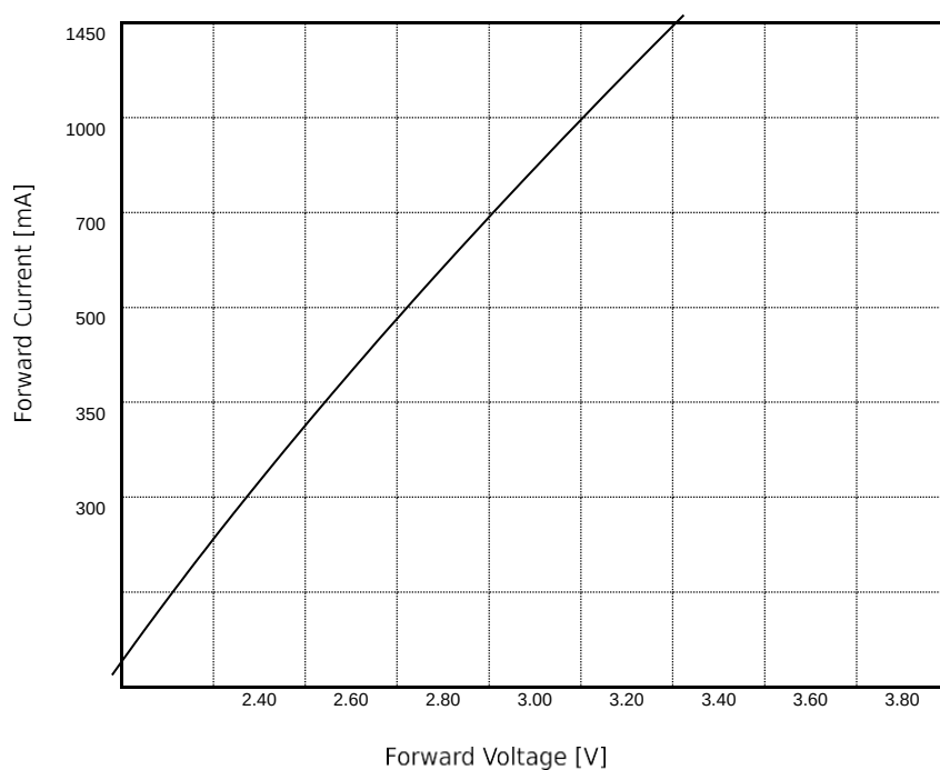
Figure 5a: Typical forward current vs. forward voltage for Queendom LED at 1000mA Tj=85°C
