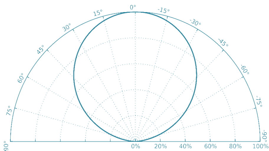
Figure 6: Typical Deg for Queendom LED at 1000mA Tj=85°C
