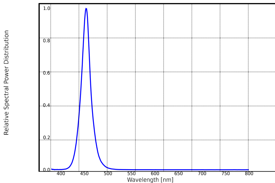
Figure 2: Typical normalized power vs. wavelength for Queendom at specified test current, T_a=25^{\circ}\text{C}
