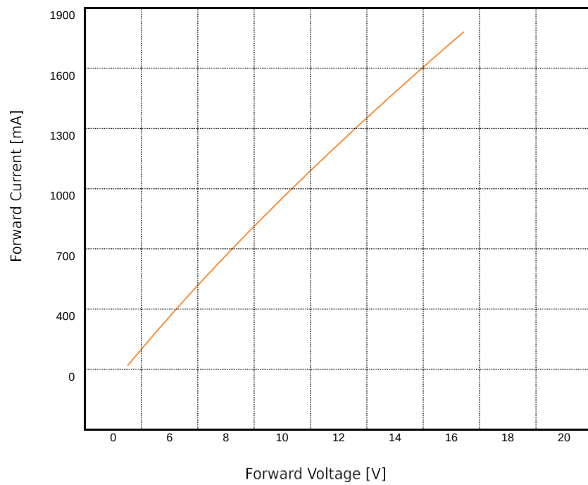
Figure 5a: Typical forward current vs. forward voltage for Queendom LED at 1000mA T_j=85^{\circ}\text{C}
