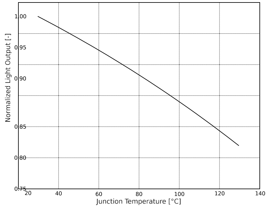
Figure 3. Typical normalized light output vs. junction temperature for at specified test current. Tj=25°C .
