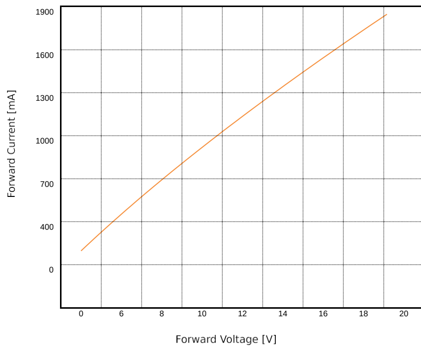
Figure 5a: Typical forward current vs. forward voltage for Queendom LED at 1500mA T_j=85^{\circ}\text{C}
