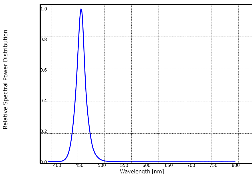
Figure 2: Typical normalized power vs. wavelength for Queendom at specified test current, T_a=25^{\circ}\text{C}
