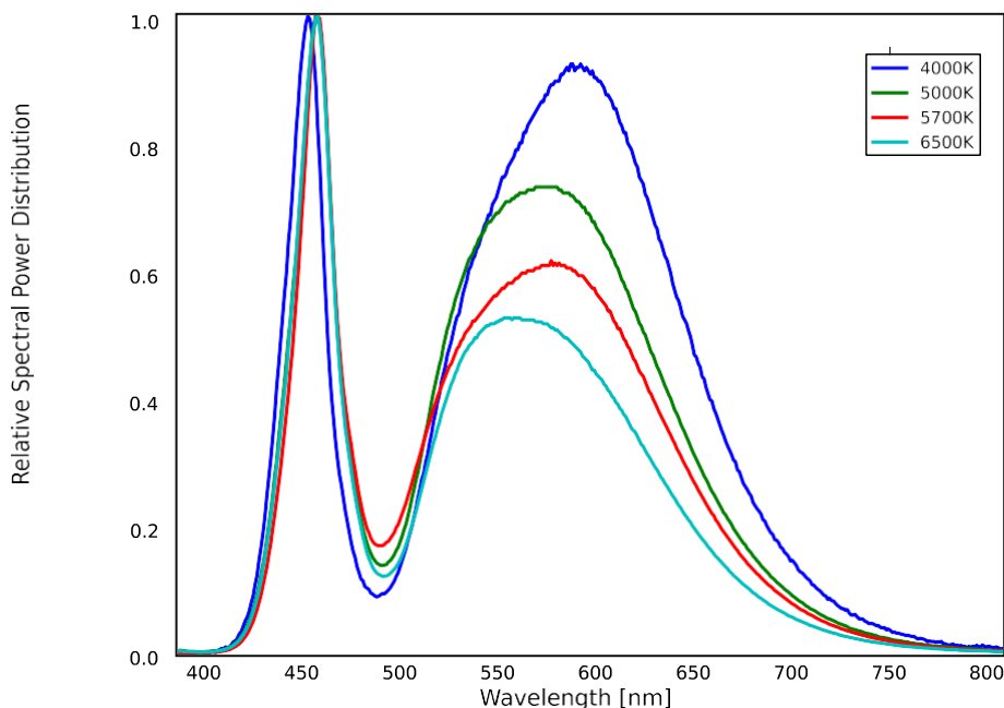
Figure 1: Typical normalized power vs. wavelength for Queendom at specified test current, T_j=85^{\circ}\text{C}
